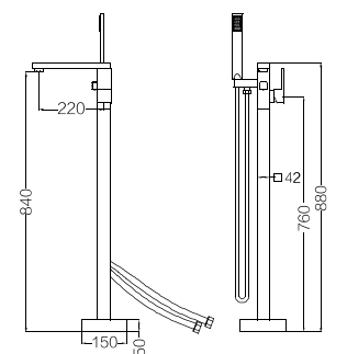
DT-1120 Bath shower floor standing mixer Material: Brass
