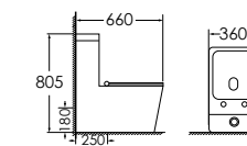
8017 Washdown one-piece toilet Size: 660x360x805 mm P-trap, 180 mm roughing-in S-trap, 250 mm roughing-in
