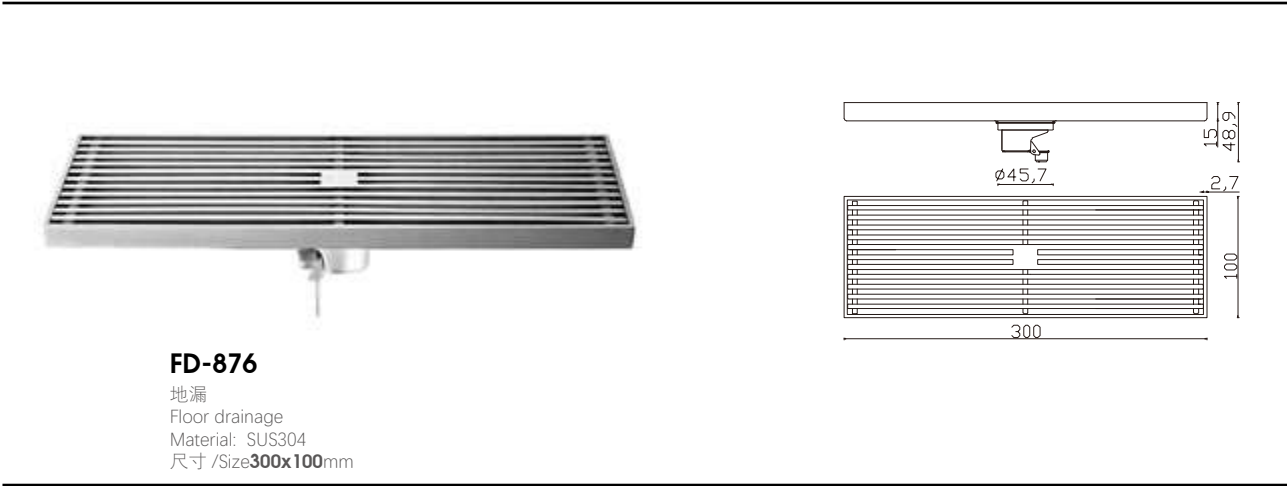
FD-875 地漏 Floor drainage Material: SUS304 尺寸 /Size 300x100 mm
