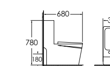
8215 Washdown one-piece toilet Size: 680x360x780 mm P-trap, 180 mm roughing-in S-trap, 250 mm roughing-in
