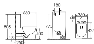
1004A Washdown one-piece toilet Size: 660x360x805 mm P-trap, 180 mm roughing-in S-trap, 250 mm roughing-in
