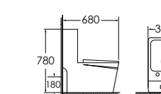
8215 Washdown one-piece toilet Size: 680x360x780 mm P-trap, 180 mm roughing-in S-trap, 250 mm roughing-in
