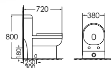
8010 Washdown one-piece toilet Size: 720x380x800 mm P-trap, 180 mm roughing-in S-trap, 250/300 mm roughing-in
