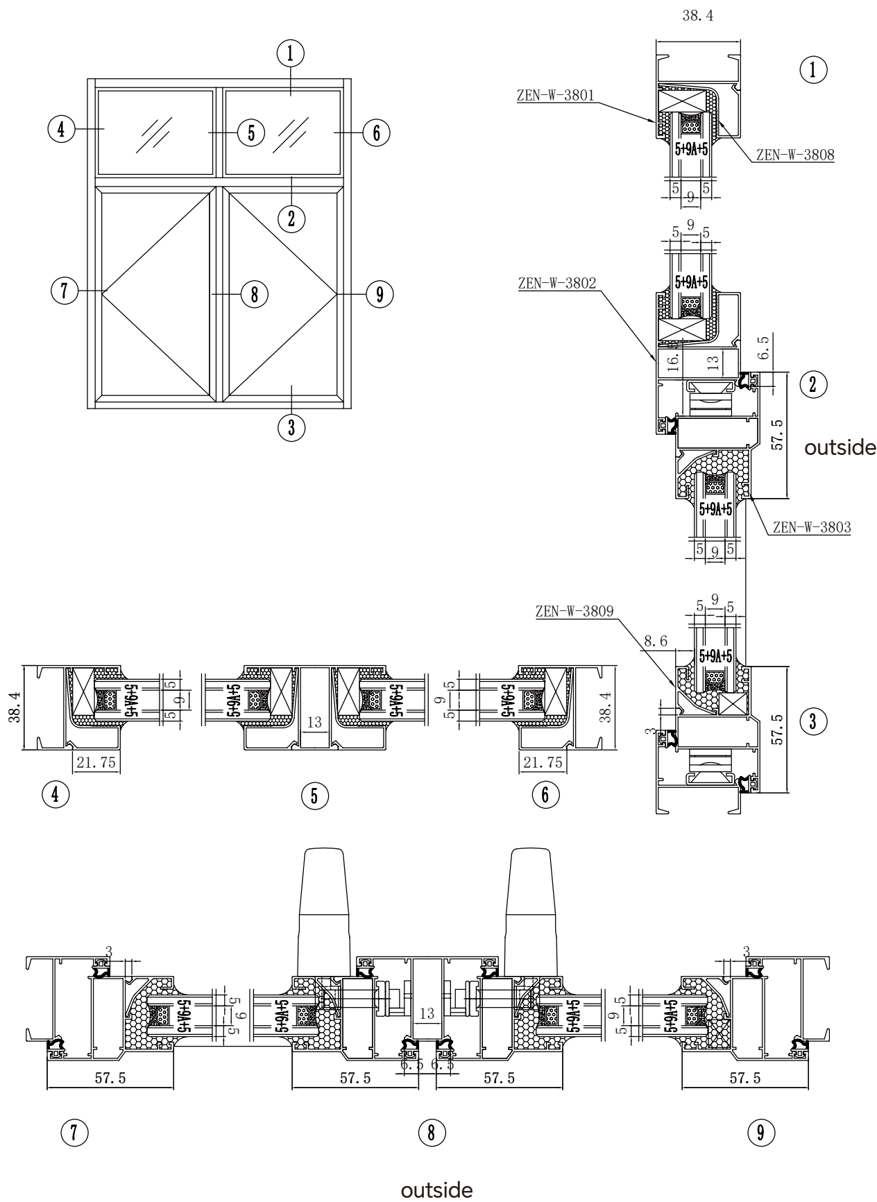
Assembly drawing of 40 series double-glazed casement windows
