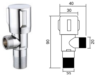
FJF-030 角阀 Angle valve Material: Brass
