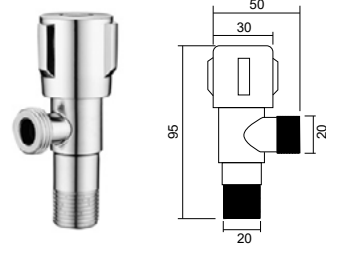
FJF-030BR 角阀 Angle valve Material: Brass
