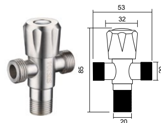
DJF-015BR 角阀 Angle valve Material: SUS304
