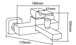
DT-1114 Shower faucet Material: Brass
