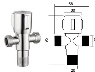
DJF-004 角阀 Angle valve Material: SUS304
