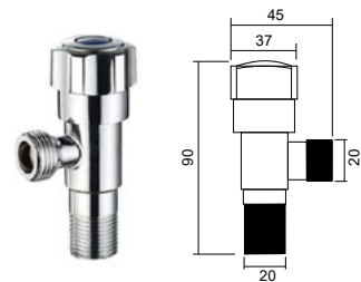
DJF-001 角阀 Angle valve Material: SUS304
