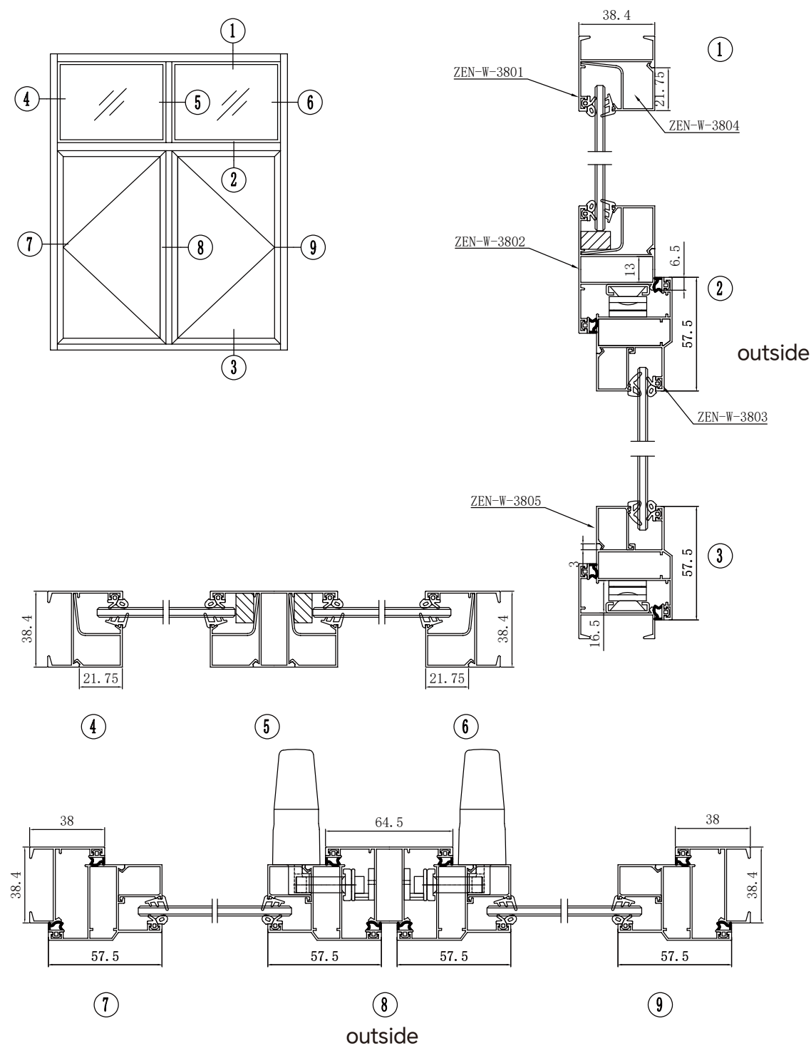
Assembly drawing of 40 series single-glazed casement windows
