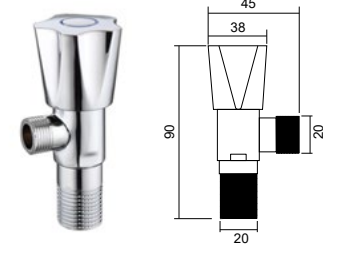
FJF-036 角阀 Angle valve Material: Brass
