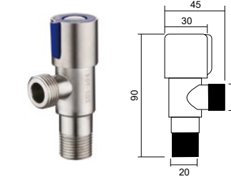
DJF-017BR 角阀 Angle valve Material: SUS304
