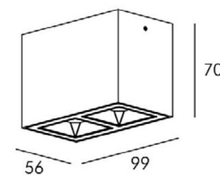
OL C78048-2/2x5w Bridgelux SMD
