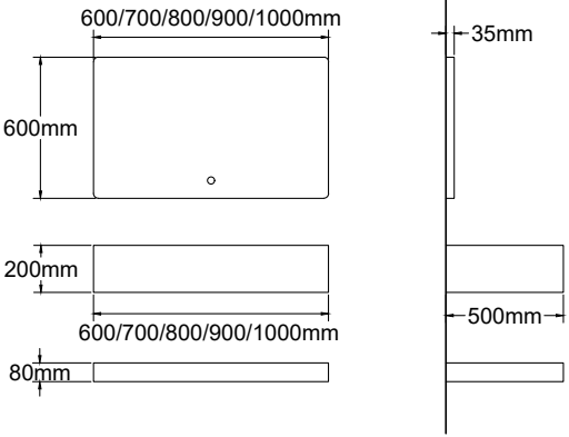
T-9070 Counter tops: 700x500x200 mm Shelf Borad: 700x500x80 mm LED Mirror: 700x600 mm Sintered Stone: Arabescato Corchia
