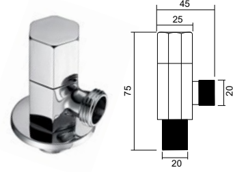
JF-012 角阀 Angle valve Material: Brass
