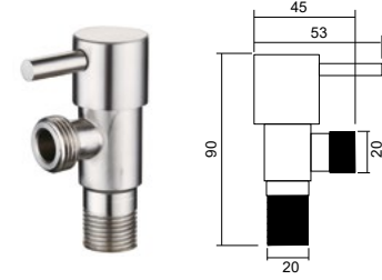
DJF-016BR 角阀 Angle valve Material: SUS304
