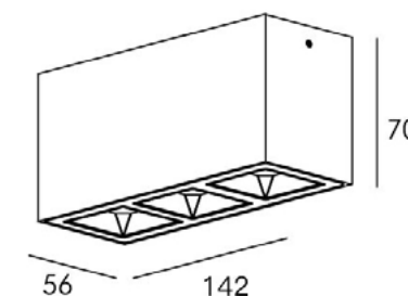
OL C78048-3/3x5w Bridgelux SMD
