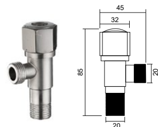
DJF-010BR 角阀 Angle valve Material: SUS304
