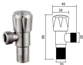
DJF-013 角阀 Angle valve Material: SUS304
