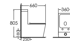
8017 Washdown one-piece toilet Size: 660x360x805 mm P-trap, 180 mm roughing-in S-trap, 250 mm roughing-in
