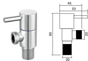
FJF-042 角阀 Angle valve Material: Brass
