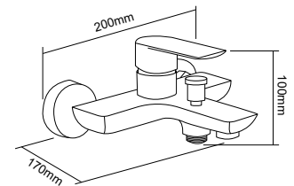
DT-0506 Shower faucet Material: Brass
