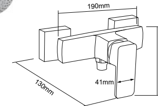
DT-1113 Shower faucet Material: Brass
