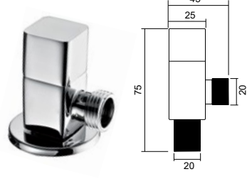
JF-047 角阀 Angle valve Material: Brass
