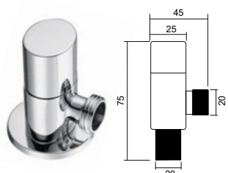
JF-046 角阀 Angle valve Material: Brass
