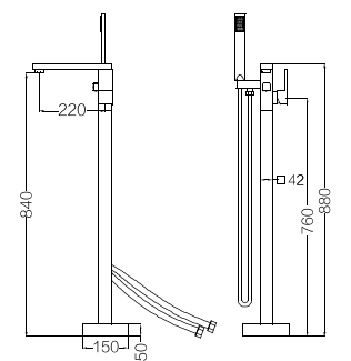
DT-1120 Bath shower floor standing mixer Material: Brass
