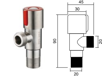
DJF-018BR 角阀 Angle valve Material: SUS304
