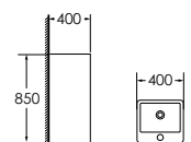
1004S Stand basin Size: 400x400x850 mm Fixing to wall with back
