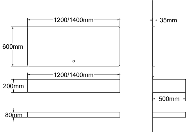
T-96120 台面 /Counter tops: 1200x500x200 mm 搁板 /Shelf Borad: 1200x500x80 mm 智能镜 /LED Mirror: 1200x600 mm 岩板 /Sintered Stone: 冰晶石 /Cryolite Glass
