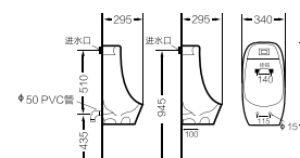
7015 挂墙式小便斗 Wall hung urinal 尺寸 /Size 340x295x680 mm 用背固定在墙上 Fixing to wall with back
