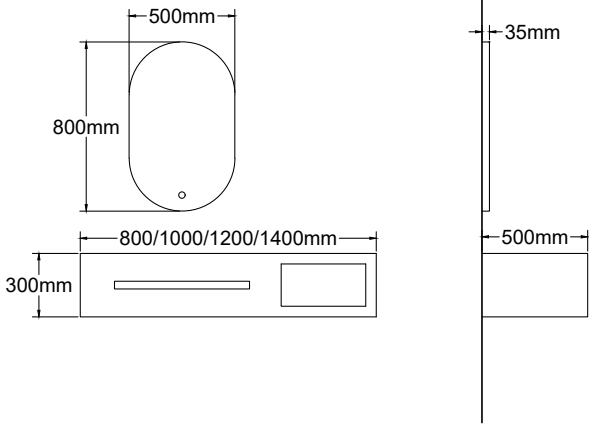
T-94140 主柜 /Main Cabinet: 1400x500x300 mm 智能镜 /LED Mirror: 500x800 mm 岩板 /Sintered Stone: 阿玛尼灰 /Armani Grey
