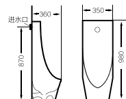
7006 落地式小便池 Floor standing urinal 尺寸 /Size 350x360x980 mm 背墙安装 Back to wall installation
