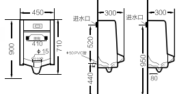
7013 挂墙式小便斗 Wall hung urinal 尺寸 /Size 450x300x710 mm 用背固定在墙上 Fixing to wall with back
