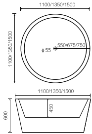
BT-054 独立式浴缸 Freestanding bathtub 尺寸 /Size: 1100x1100x600mm 1350x1350x600mm 1500x1500x600mm
