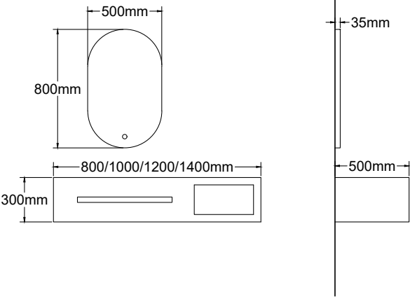
T-97140 主柜 /Main Cabinet: 1400x500x300 mm 智能镜 /LED Mirror: 500x800 mm 岩板 /Sintered Stone: 冰晶石 /Cryolite Glass
