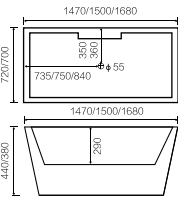
BT-065 独立式浴缸 Freestanding bathtub 尺寸 /Size: 1470x720x440mm 1500x700x380mm 1680x720x440mm
