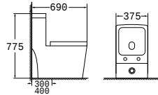
8108 虹吸连体马桶 Siphonic one-piece toilet 尺寸 /Size: 690x375x775 mm 地排 /S-trap, 300/400 mm roughing-in
