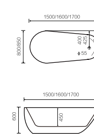
BT-020 独立式浴缸 Freestanding bathtub 尺寸 /Size: 1500x800x600mm 1600x800x600mm 1700x850x600mm
