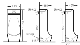
7001 落地式小便池 Floor standing urinal 尺寸 /Size 410x455x1020 mm 背墙安装 Back to wall installation
