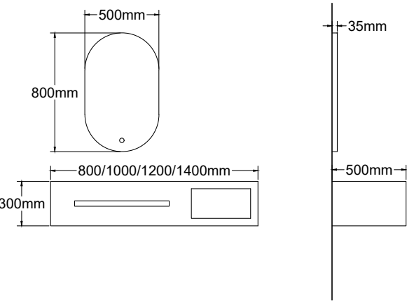
T-91140 主柜 /Main Cabinet: 1400x500x300 mm 智能镜 /LED Mirror: 500x800 mm 岩板 /Sintered Stone: 鱼肚白 /Arabescato Corchia
