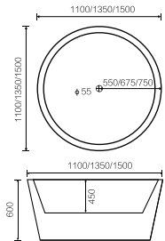
BT-054B 独立式浴缸 Freestanding bathtub 尺寸 /Size: 1100x1100x600mm 1350x1350x600mm 1500x1500x600mm
