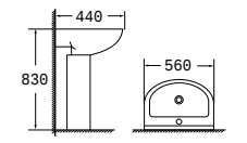
1023B 分体柱盆 Pedestal basin 尺寸 /Size: 560x440x830 mm 用背固定在墙上 Fixing to wall with back
