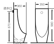
7006 落地式小便池 Floor standing urinal 尺寸 /Size 350x360x980 mm 背墙安装 Back to wall installation
