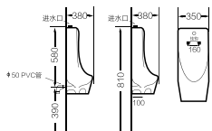
7009 挂墙式小便斗 Wall hung urinal 尺寸 /Size 380x350x760 mm 用背固定在墙上 Fixing to wall with back
