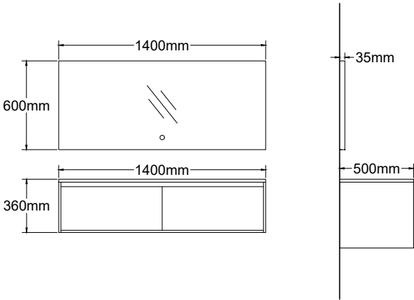
F-5072 LED 主柜 /Main Cabinet: 1400x500 mm 镜子 /Mirror : 1400x600 mm 岩板 /Sintered Stonet: 鱼肚白 /Arabescato Corchia 材质 /Plywood
