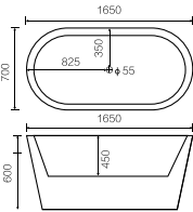
BT-060 独立式浴缸 Freestanding bathtub 尺寸 /Size: 1650x700x600mm
