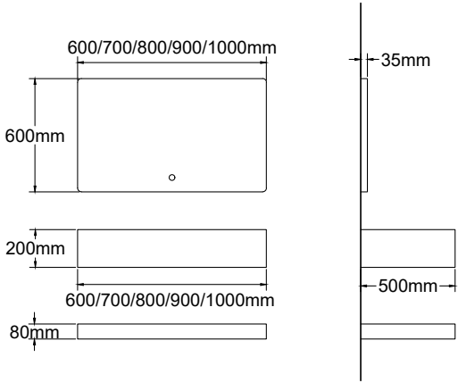
T-9070 台面 /Counter tops: 700x500x200 mm 搁板 /Shelf Borad: 700x500x80 mm 智能镜 /LED Mirror: 700x600 mm 岩板 /Sintered Stone: 鱼肚白 /Arabescato Corchia
