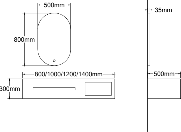
T-94140 主柜 /Main Cabinet: 1400x500x300 mm 智能镜 /LED Mirror: 500x800 mm 岩板 /Sintered Stone: 阿玛尼灰 /Armani Grey
