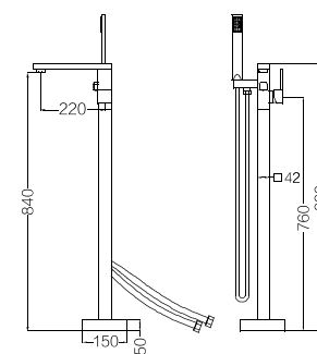
DT-1120 落地式浴缸淋浴龙头 Bath shower floor standing mixer 材料 /Material: A 级铜 /Brass
