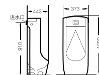
7003 落地式小便池 Floor standing urinal 尺寸 /Size 443x373x1000 mm 背墙安装 Back to wall installation
