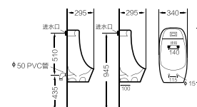
7015 挂墙式小便斗 Wall hung urinal 尺寸 /Size 340x295x680 mm 用背固定在墙上 Fixing to wall with back
