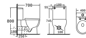
1023A 直冲分体马桶 Washdown two-piece toilet 尺寸 /Size: 700x400x800 mm 墙排 /P-trap, 180 mm roughing-in 地排 /S-trap, 250 mm roughing-in
