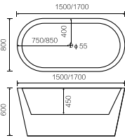
BT-008 独立式浴缸 Freestanding bathtub 尺寸 /Size: 1500x800x600mm 1700x800x600mm
