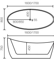
BT-023 独立式浴缸 Freestanding bathtub 尺寸 /Size: 1600x800x750 mm 1700x800x750 mm
