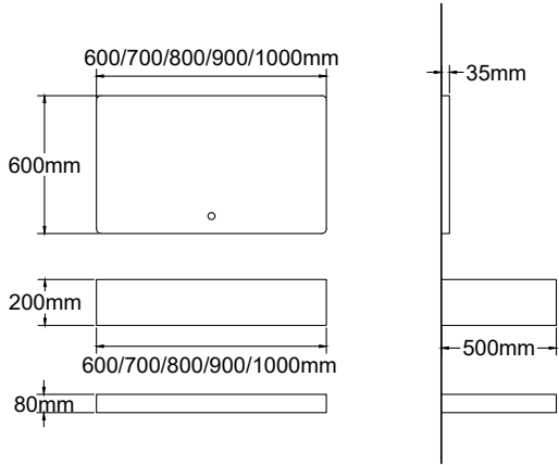
T-10570 台面 /Counter tops: 700x500x200 mm 搁板 /Shelf Borad: 700x500x80 mm 智能镜 /LED Mirror: 700x600 mm 岩板 /Sintered Stone: 意大利浅灰 /Italy Light Grey
