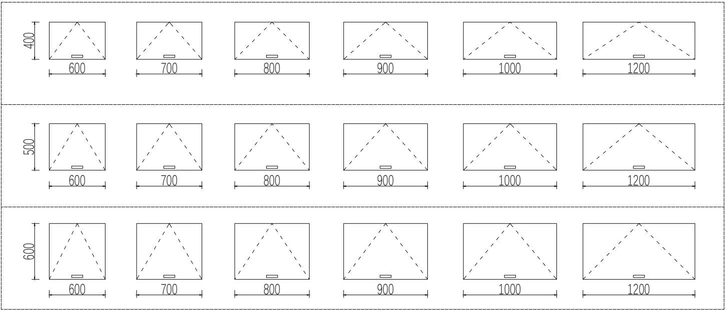
上翻门柜 Single Door Corner Floor Cabinet
