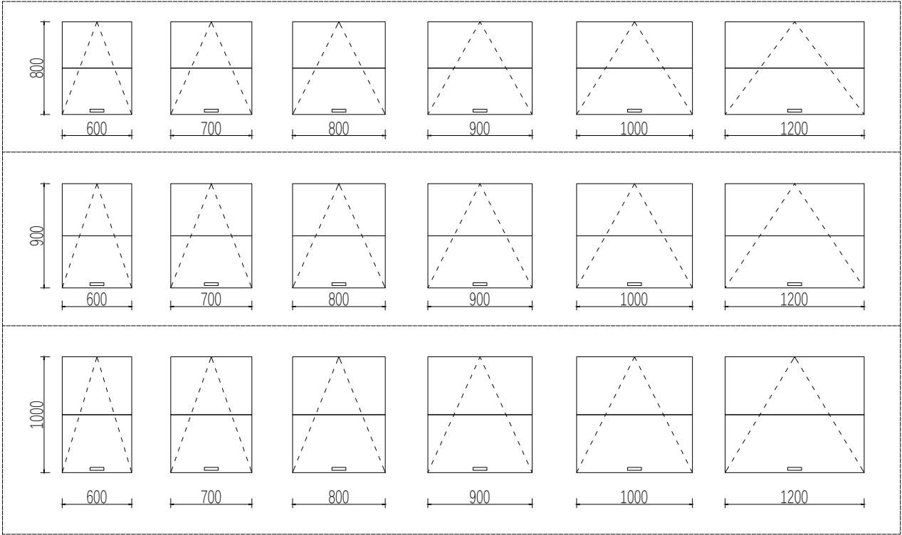
折叠上翻门柜 Fold-up Lift Door Cabinet
