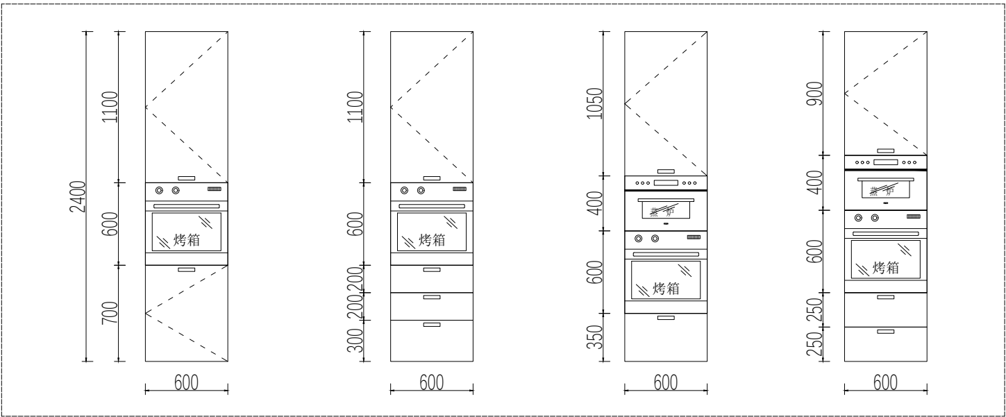
电器组合高柜 Appliance Integration Tall Cabinet
